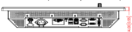
BOTTOM VIEW (without Expansion Board)
